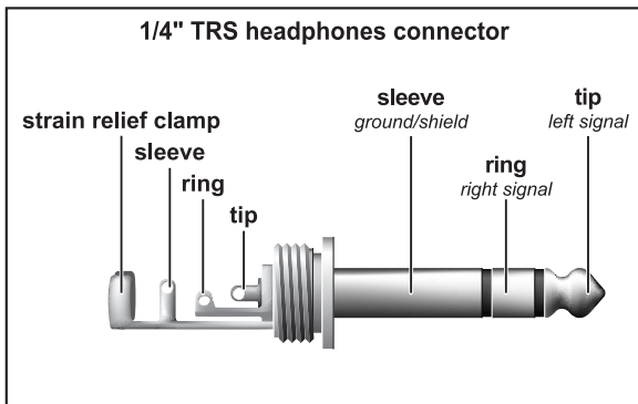
4.2: Wiring of a stereo headphones plug
